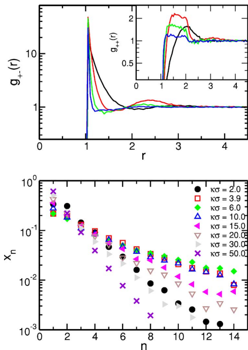
FIG. 5. Upper panel: partial pair distribution functions for T^*=0.18 and \rho^*=0.05 with \kappa=2 (black curve), \kappa=6 (red curve), \kappa=15 (green curve), and \kappa=30 (blue curve); opposite sign (main figure) and same sign (inset). Lower panel: fraction of particles in a cluster with n particles for the same state and different \kappa as labeled. x_n is normalized as \sum x_n=1 .
