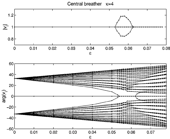
FIG. 6. Evolution of the monodromy eigenvalues with the coupling \epsilon , for the central breather. Top: modulus; bottom: arguments. The points are the calculated eigenvalues, the lines are guides to the eye.
