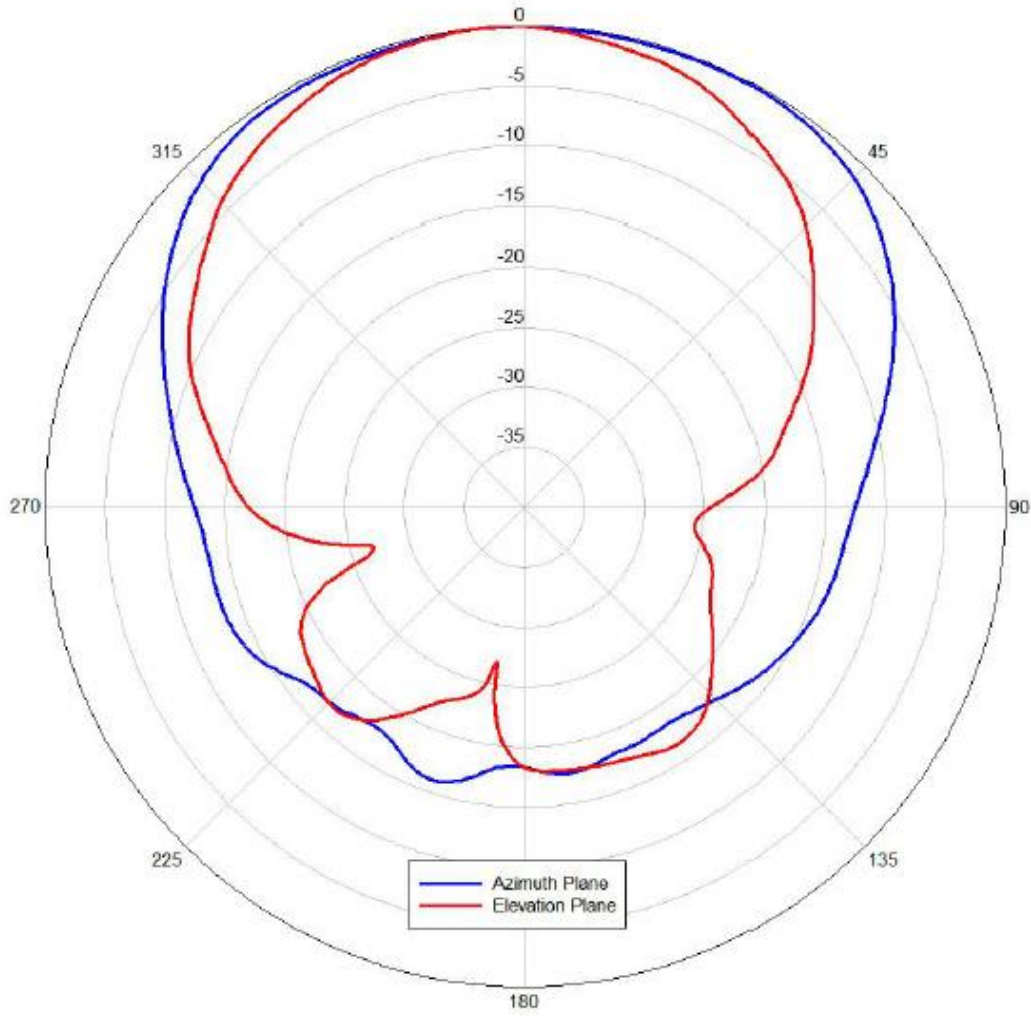
Figure 1 Azimuth and Elevation Radiation Patterns - 2.4 GHz Band
