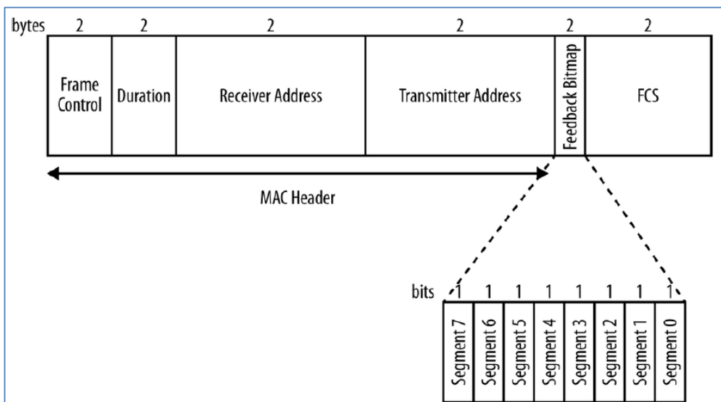
Figura 5-13 Trama Beamforming Report Poll
