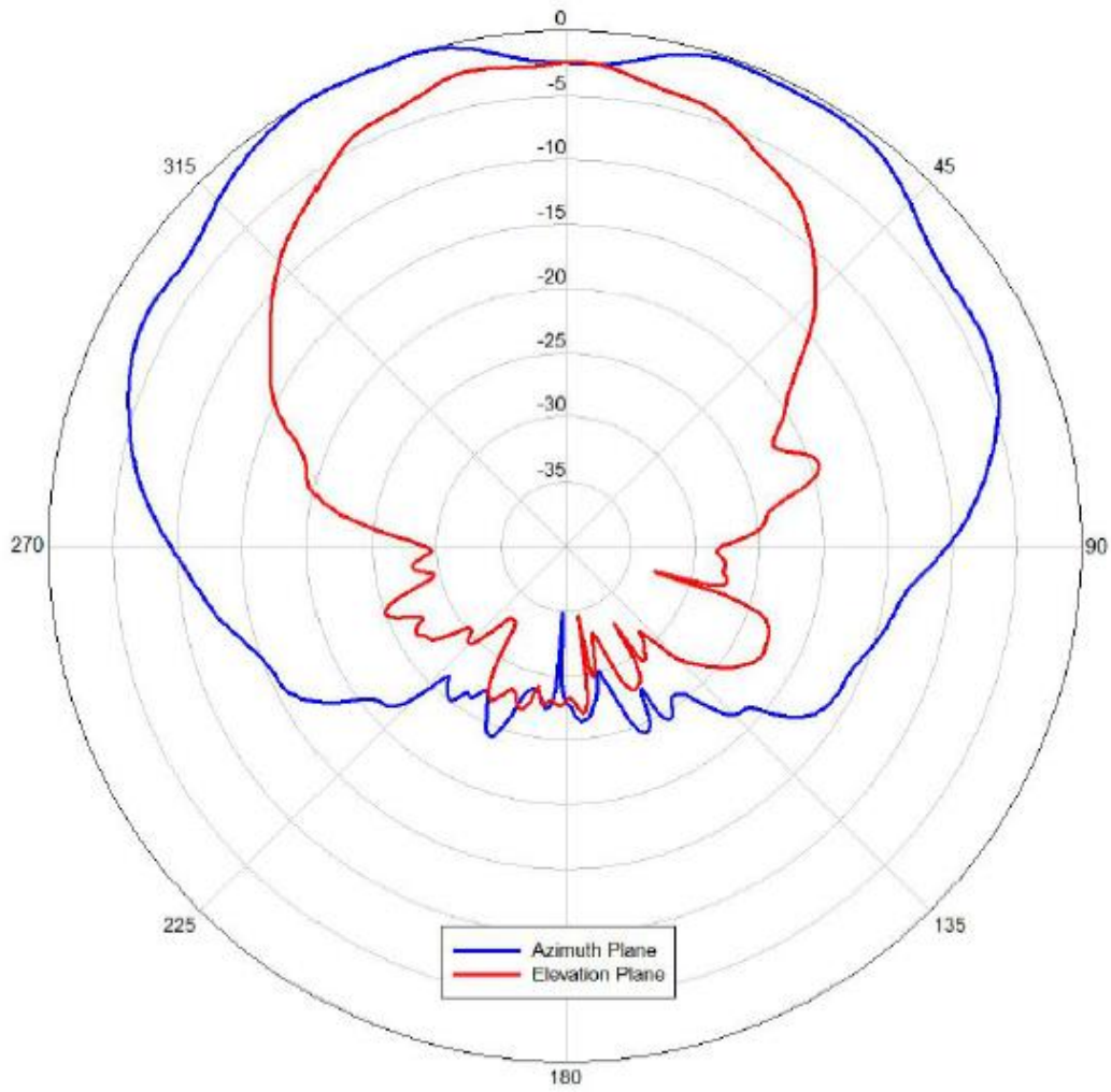
Figure 2 Azimuth and Elevation Radiation Patterns - 5 GHz Band
