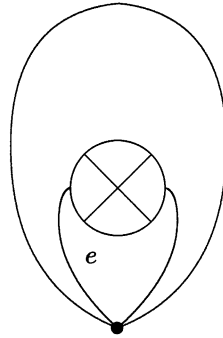
Fig. 2. Self-incident edge e .
