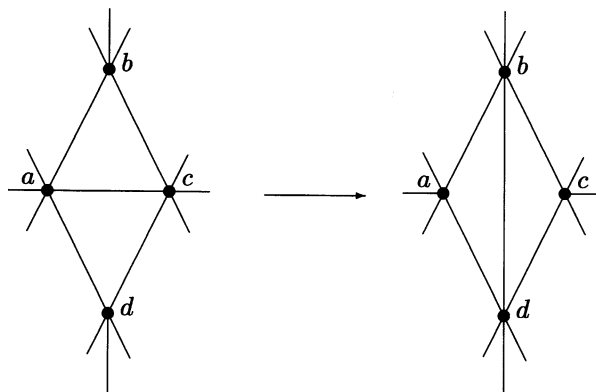
Fig. 1. A diagonal flip.
