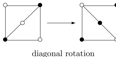
Figure 2: Diagonal transformations on quadrangulations.
