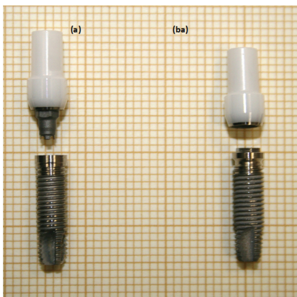
Fig. 1. Dental structures used in this study: ZiReal zirconia abutments and Osseotite titanium implants with (a) internal and (b) external connections.
