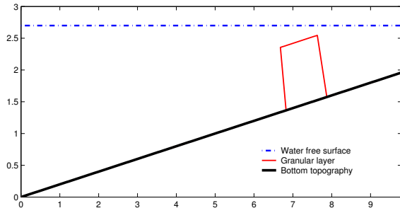
(a) Initial condition 0.0 s.
