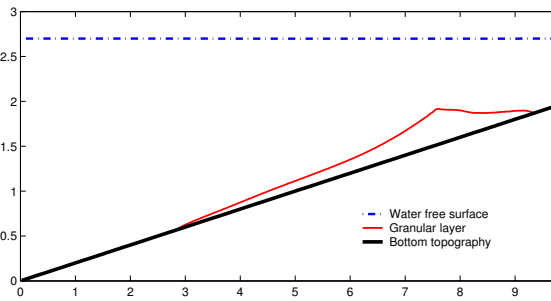
(f) 5 s. Steady state (granular material)
