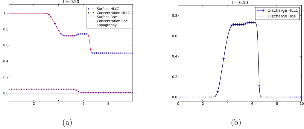
Figure 5: Simulation over flat topography
