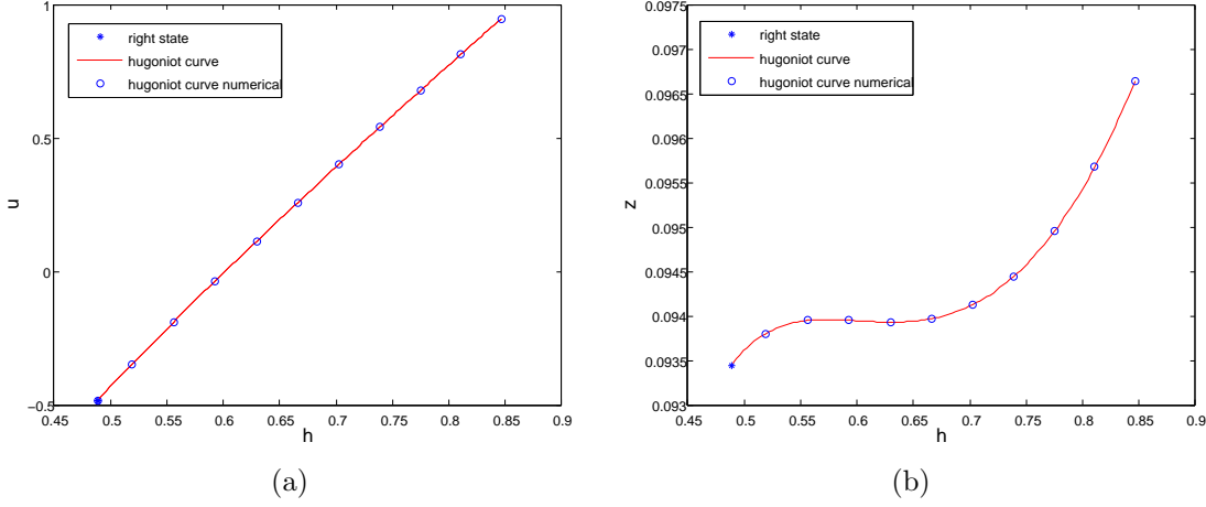
Figure 17: Hugoniot curves for external shock
