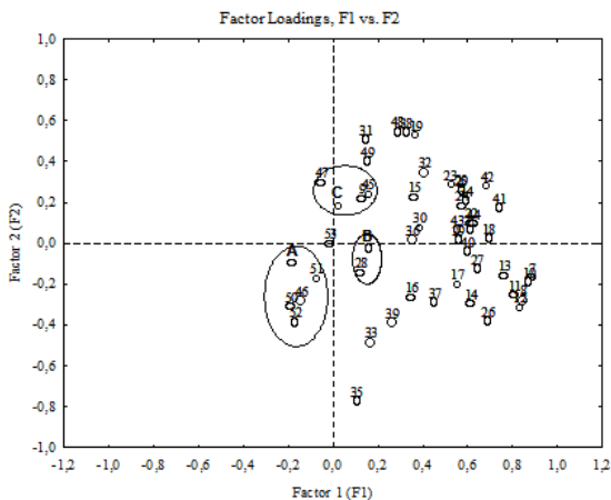
Figure 3 Results of the principal component analysis in Menorca male horses (n=200) The ellipses showed the most closely correlated traits with the three performance aptitude groups. Factor coordinates are shown, where: F corresponds to Factor 1 or 2, respectively.
