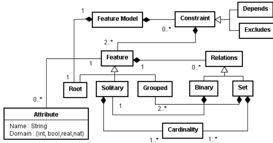
Fig. 2. FM metamodel [7]
