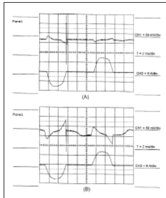
Fig. 12: Oscillograms of the voltage measure in the power transformer, using a near magnetic field probe, for the symmetrical half wave rectifier with different kind of diodes (D1 standard diode and D2 fast diodes). a) Using a 300VA transformer based on a toroidal core. b) Using a 300VA transformer based on a E-I core.
