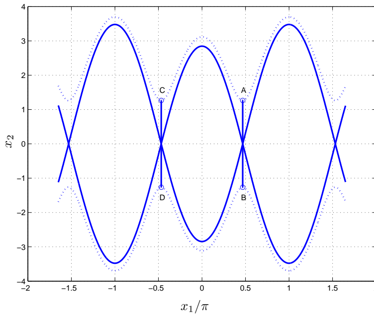
Figure 4. Level curves H_d = H^* (solid) and H_d = H^* + \varepsilon (dotted).
