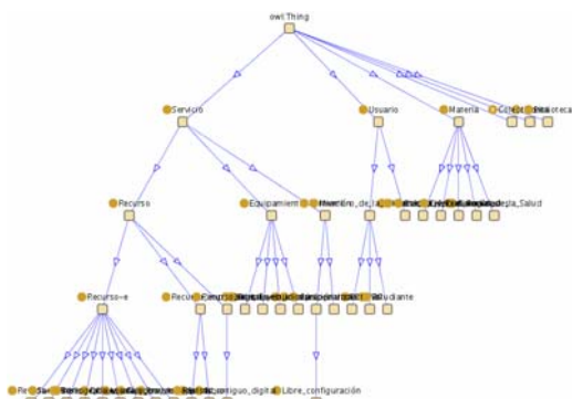
Figure 2: Class hierarchy for the OntoFama ontology
