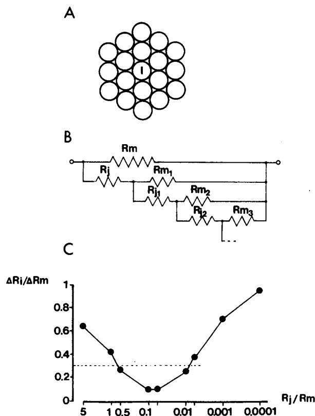
FIGURE 11. Cell-to-cell coupling in the parathyroid gland. A shows a model of cell topology in the parathyroid gland. The impaled cell (I) is surrounded by spherical shells of closely packed cells. The first, second, and third shells contain 25, 97, and 216 cells. B shows the equivalent electrical circuit of this model. R_m is the membrane resistance of a single cell, and R_j is the parallel resistance of the junctions to all of its neighbors. R_{m1} , R_{m2} , and R_{m3} are the parallel membrane resistance of the first, second, and third shell surrounding the penetrated cell and are, respectively, R_m/25 , R_m/97 , and R_m/216 . R_{j1} and R_{j2} are the resultant junctional resistance between the first and the second shells and between the second and the third shells. These values are 25R_j/97 and 25R_j/216 , respectively. C illustrates that the ratio of the change in input resistance to the change in input resistance to the change in membrane resistance ( R_i/R_m ) depends on the ratio R_j/R_m (abscissa). The interrupted line is drawn at a ratio R_i/R_m of 0.3 (a given change in R_m results in a change in R_i that is smaller by a factor of 0.33).
