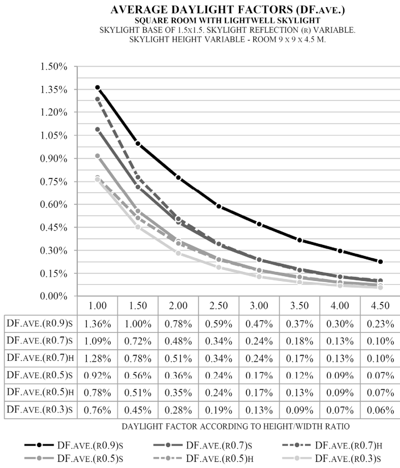
Figure 5: Trial 2: Average daylight factors (DF.ave.) on the work plane according to simulation software (S) and hypothesis (H). Variable reflection index and height of the skylight.
