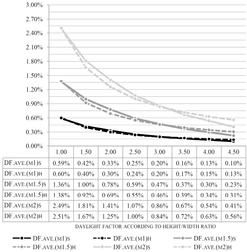
Figure 3: Trial 1: Average daylight factors (DF.ave.) on the work plane according to simulation software (S) and hypothesis (H). Variable size and ratio of the skylight.
