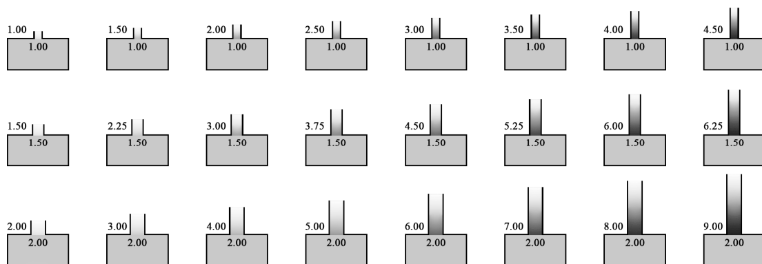
Figure 2: Trial 1: Variation in size and height/width ratio of the lightwell skylights.
