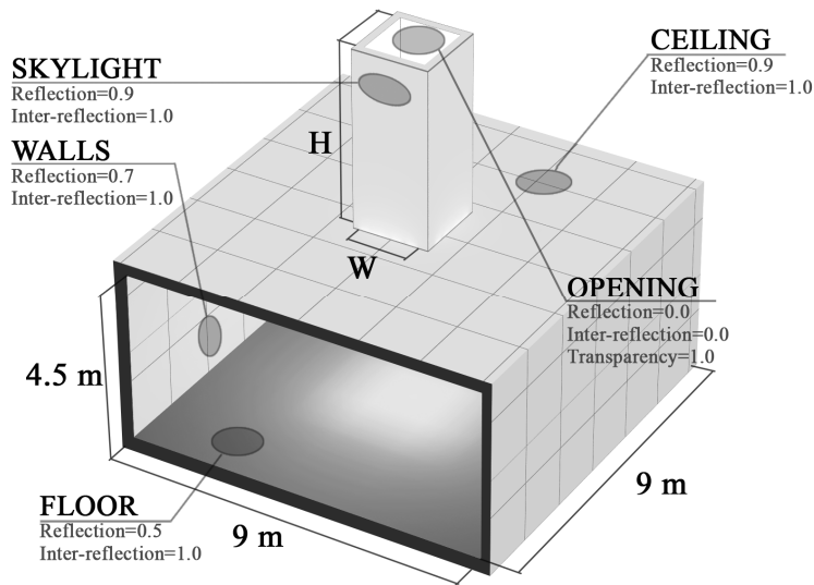
Figure 1: Initial calculation model.
