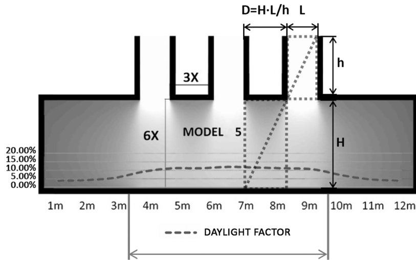
Figure 8: Trial 4: Skylight spacing according to width/height ratio of the lightwell.
