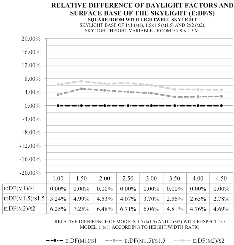
Figure 4: Trial 1: Relative difference of the quotient of average daylight factors on the work plane and the surface base of the skylight, according to simulation software. Models 1.5 (M1.5) and 2 (M2) with respect to model 1 (M1). Variable size and ratio of the skylight.
