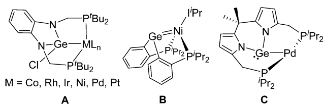
Fig. 1 Representative examples of PGeP-based transition metal complexes ( i Pr = 1,3-diisopropyl-4,5-dimethylimidazol-2-ylidene).
