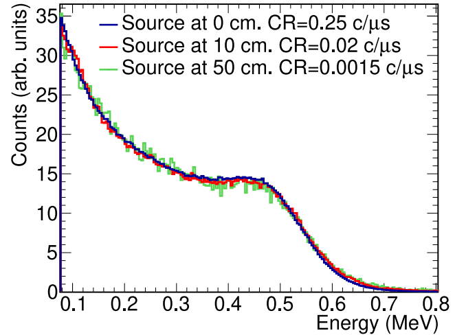
Fig. 12. Deposited energy spectra for a 20 MBq ^{137}\text{Cs} calibration source placed at different distances from an sTED module with an R11265U-100 photomultiplier, along with the Counting Rates (CR) obtained using a deposited energy threshold of 0.15 MeV.
