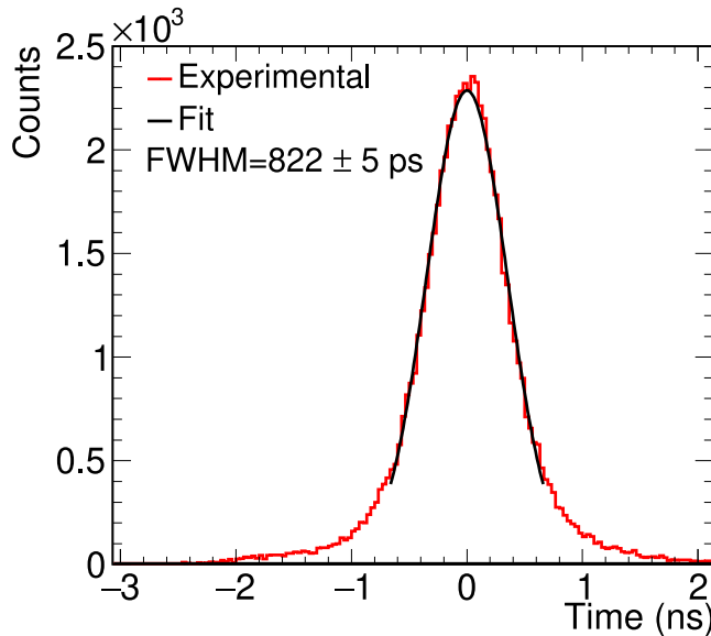
Fig. 11. Distribution of the time differences between signals in coincidence between an sTED module and a \text{LaBr}_3 detector, when measuring a ^{60}\text{Co} source. The FWHM of the distribution is 822 \pm 5 ps, including the contribution of the \text{LaBr}_3 and the sTED, see text for details.
