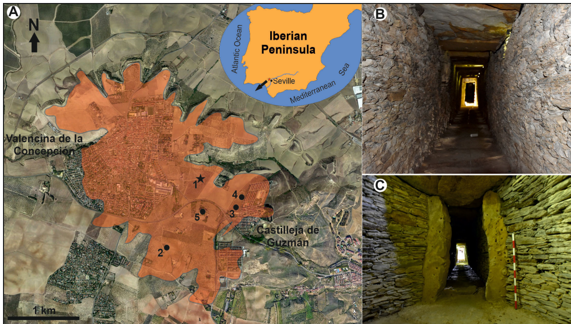
Figure 1. (A): Location and extent (brown) of the Valencina mega-site and position of its main megalithic monuments: 1: La Pastora; 2: Matarrubilla; 3: Montelirio; 4: Structure 10.042–10.049; 5: Ontiveros (background image by Google Earth). (B,C): Views of the interior of La Pastora tholos: from the access towards the interior (B) and from the chamber towards the corridor (C).
