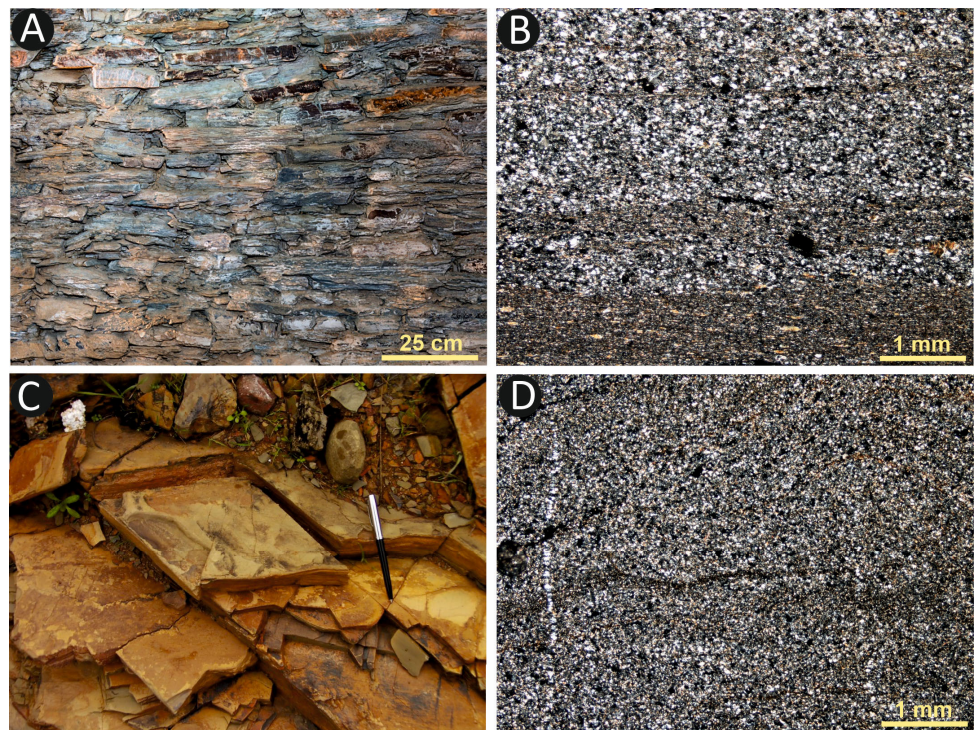
Figure 4. Quartzarenite. (A): Blocks of this lithology as masonry in the walls of La Pastora. (B): A representative thin-section photomicrograph of a block from the monument. (C): Outcrop of the PQ formation in the Cuesta de la Media Fanega area. (D): A thin section of quartzarenites in the latter outcrop.
