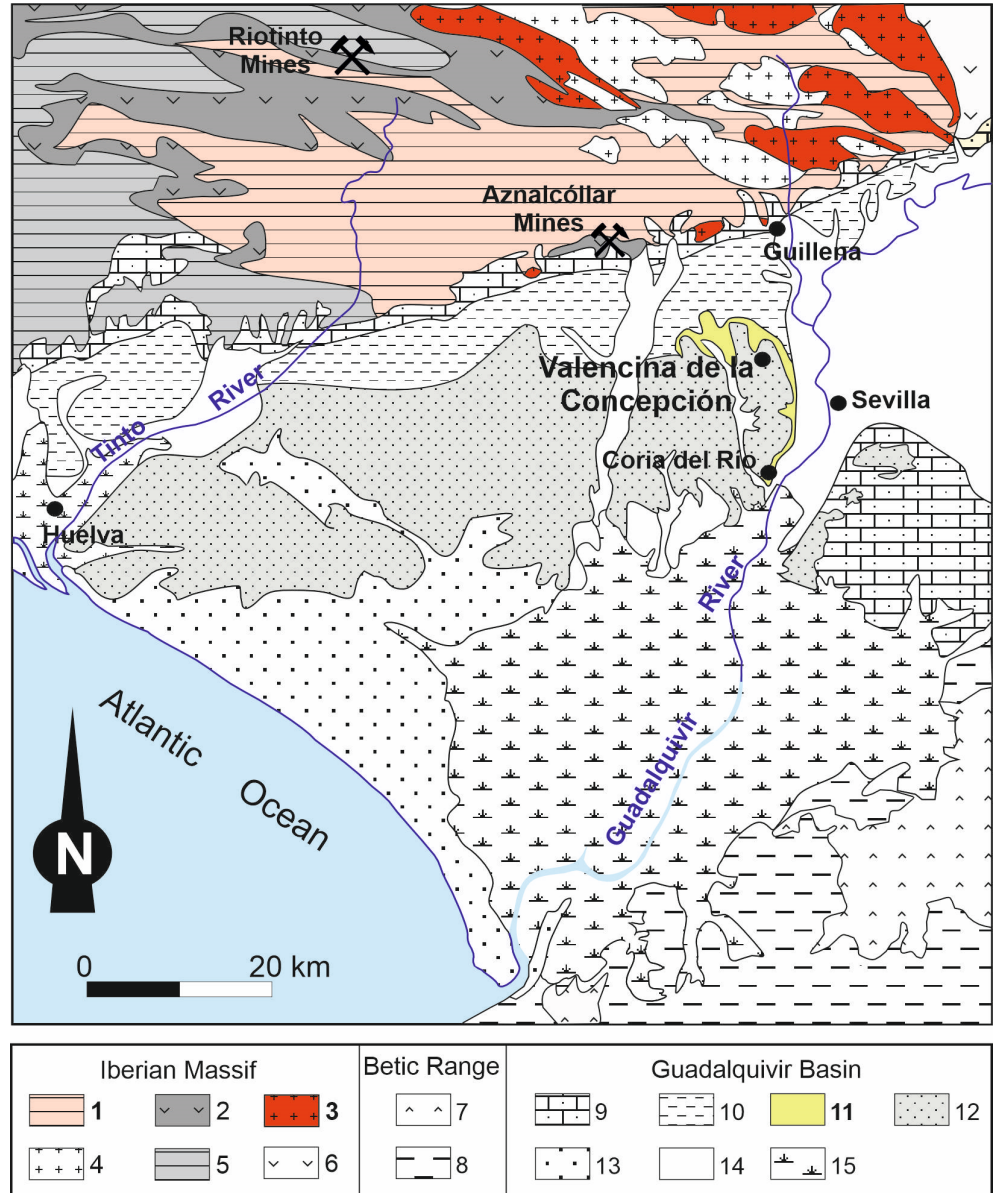
Figure 3. Geological setting of the southwest of the Iberian Peninsula, around the Valencina mega-site. Key: 1: Devonian quartzarenites and shales, the PQ Group; 2: Carboniferous Volcanic Sedimentary Complex; 3: Granitoid (SNSB); 4: Basic plutonic rocks (SNSB); 5: Carboniferous greywackes and shales, the Culm Group; 6: Permian volcanic and sedimentary rock (PVB); 7: Triassic clay and gypsum; 8: Miocene marl, sandstone, and flint stone; 9: Tortonian sandstone and conglomerate; 10: Miocene marl, Blue Marl Unit; 11: Transition Facies; 12: Pliocene sand and silt; 13: Quaternary sand (dunes and beaches); 14: Quaternary fluvial deposits (conglomerate, sand, and clay); and 15: marshland. In color, the geological formations from which the stones of La Pastora tholos come (modified from [7]).
