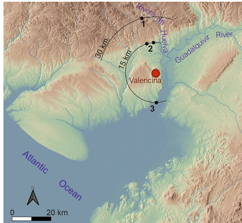
Figure 8. Map showing the approximate situation of the area around Valencina in the third millennium BC. Location of the possible areas of provenance of the rocks of La Pastora with distances to the Valencina mega-site: 1: Cuesta de la Media Fanega. 2: Gerena (west point) and Guillena (east point). 3: Coria del Río. (map art by Francisco Sánchez Díaz).
