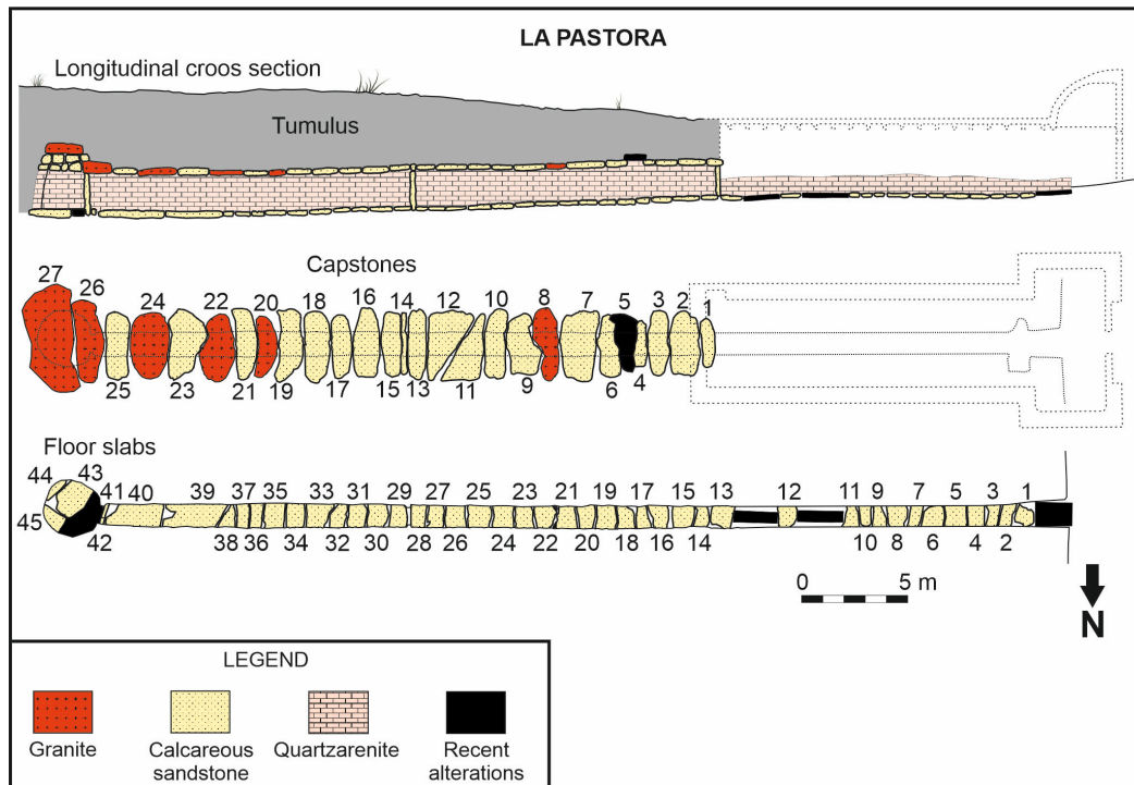
Figure 2. La Pastora section, capstones, and floor plans, with the lithology of their constructive elements and numbering of capstones and floor slabs of the monument ordered from the entrance to the chamber. (modified from [8]).
