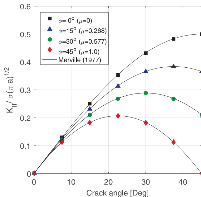
Fig. 8 Numerical results vs. analytical solutions for normalized K_{II} ( K_{II}/\sigma\sqrt{\pi a} ) for various inclination angles ( \alpha ) and different friction angles ( \phi ).
