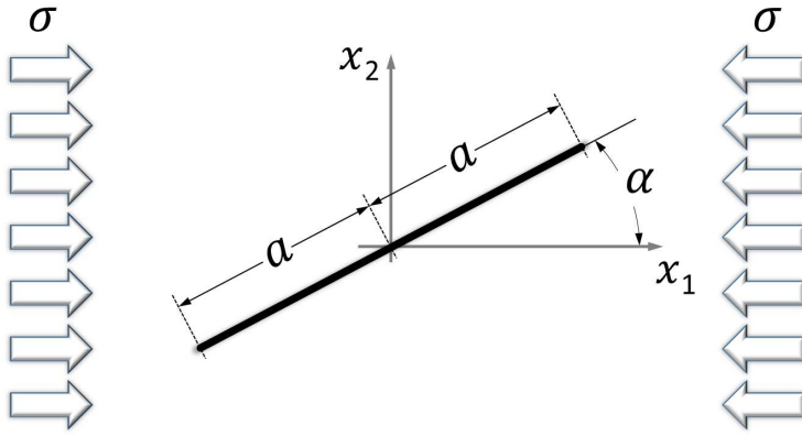
Fig. 7 A crack under compression in an unbounded domain.
