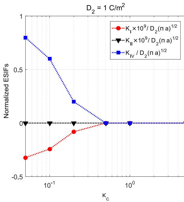
Fig. 6 Influence of the permittivity parameter \kappa_c on the intensity factors K_I , K_{II} and K_{IV} for the uniform electric displacements loading D_2 = 1 \text{ C/m}^2 .
