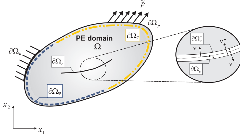
Fig. 1 Fractured piezoelectric domain.
