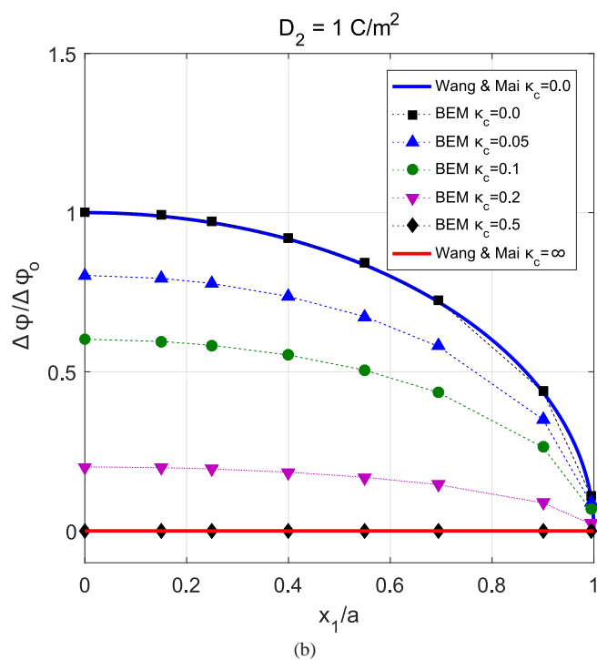
Fig. 3 Influence of the permittivity parameter \kappa_c on: (a) the crack opening displacements and (b) the electric potential increment along the crack due to an uniform electric displacements loading: D_2 = 1 \text{ C/m}^2 .
