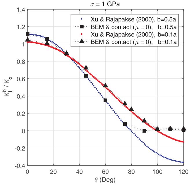
Fig. 11 Normalized stress intensity factors K_I at the tip of a branched crack due to remote tension: K_I^b/K_o , being K_o = \sigma\sqrt{\pi a} . Comparison between the boundary element solution including frictionless ( \mu = 0 ) contact and the analytical solution from [21] for different branched crack orientation angles ( \theta ) and branch lengths ( b ).
