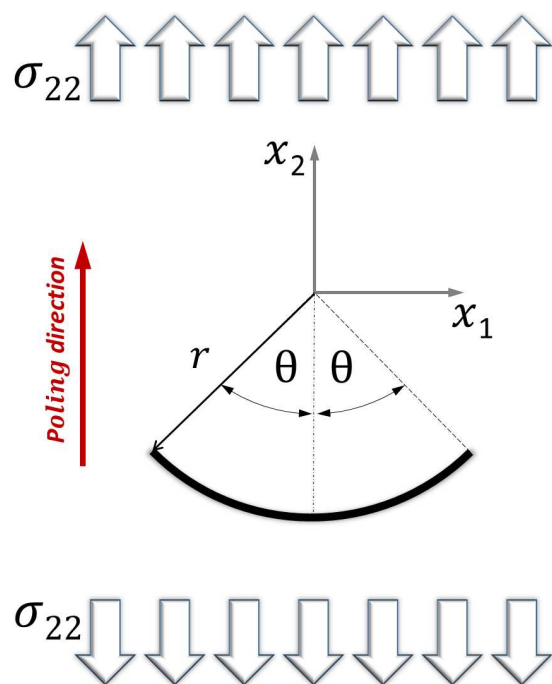
Fig. 13 Curved crack in unbounded domain.
