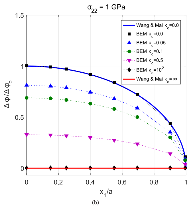
Fig. 4 Influence of the permittivity parameter \kappa_c on: (a) the crack opening displacements and (b) the electric potential increment along the crack for uniform traction loading: \sigma_{22} = 1 \text{ GPa} .
