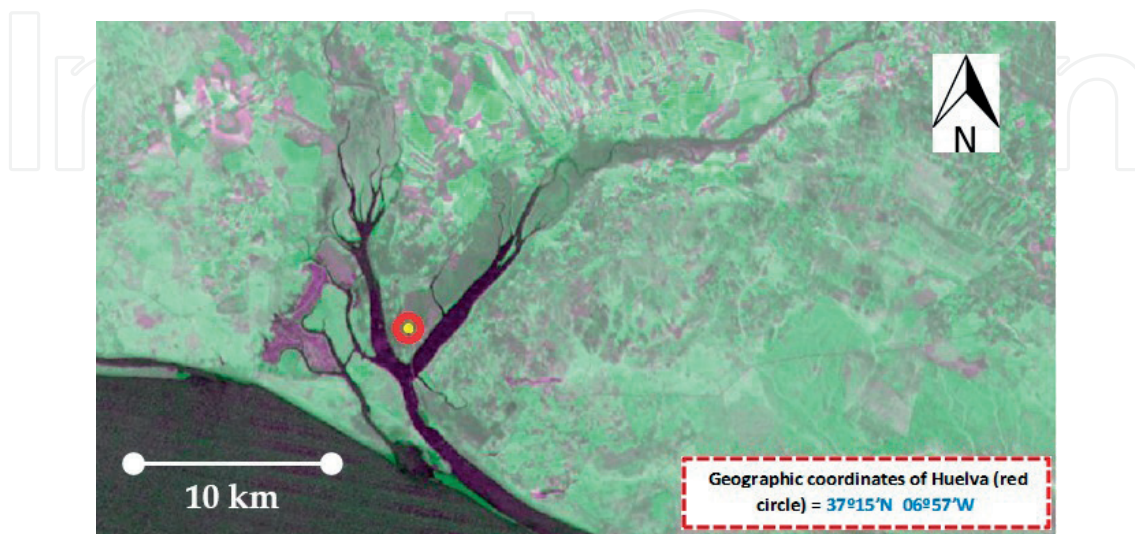
Figure 4. Detected changes in study area between 1975 and 1990.
