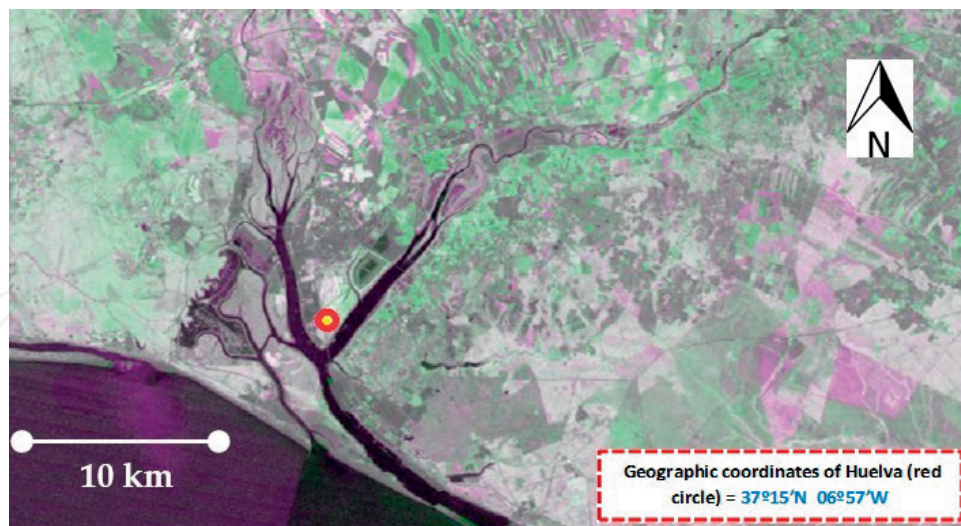
Figure 7. Detected changes in study area between 2005 and 2012.
