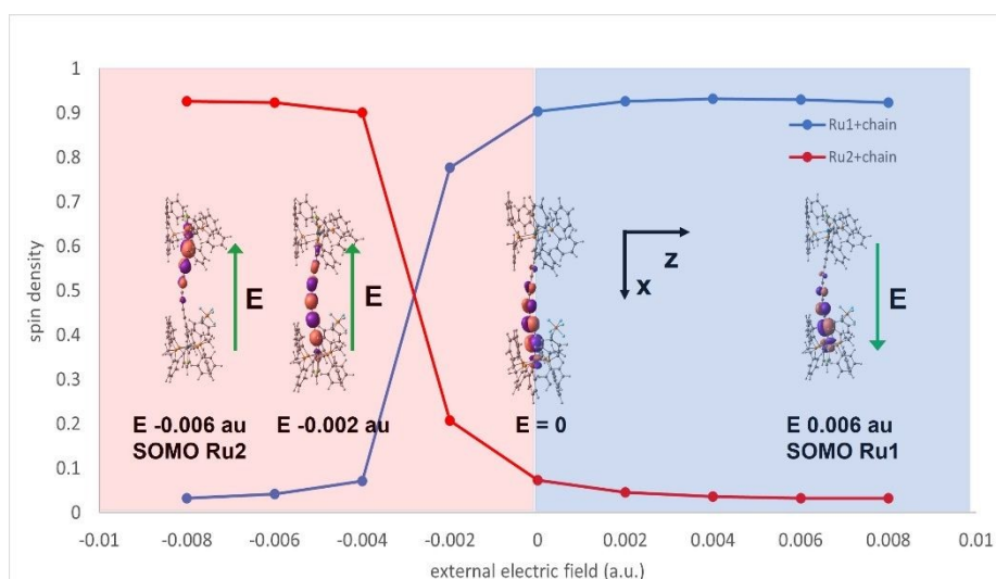
Figure 6. Response curve of the \text{Ru}2^+ molecule under an applied electric field (in atomic units, 1 \text{ au} = 51.4 \text{ V \AA}^{-1} ) along the long axis of the molecule. Blue (red) area corresponds to positive (negative) electric fields. The insets show the shape of the singly occupied orbital of the dominant configuration of the ground state CASSCF(7/4) wavefunction.
