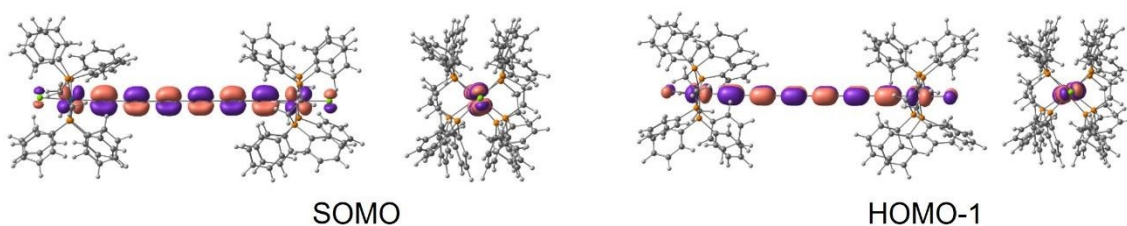
Figure 4. Front and side views of the (left) SOMO and (right) HOMO-1 orbitals for the isolated Ru2 + molecule at B3LYP* level, similar for the rPBE description.
