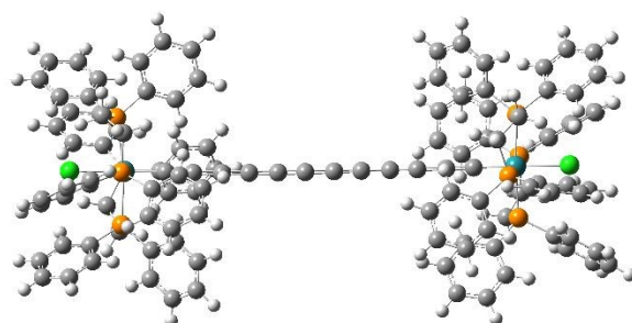
Figure 2. Representation of the Ru2 molecule: dark green, grey, white, orange and light green correspond to Ru, C, H, P and Cl, respectively.
