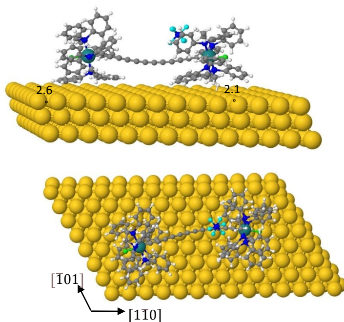
Figure 5 Top and side views of the Ru 2 + molecule and PF 6 - ion deposited on Au(111) surface. Au, Ru, C, F, Cl, P and H are represented by yellow, green, grey, cyan, light green, blue and white balls, respectively.
