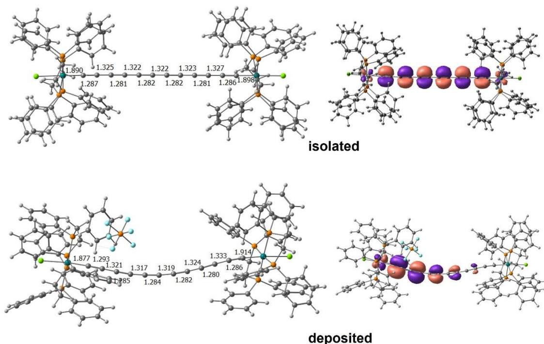
Figure 3. (left) C-C and C-Ru bond distances in Ru 2 + molecule from rPBE calculations on the optimized geometries for the isolated (top) and deposited molecule on Au(111) in presence of the PF 6 - counterion (bottom). (right) Singly occupied orbitals of the lowest doublet state from state average CASSCF(7/4) calculations.
