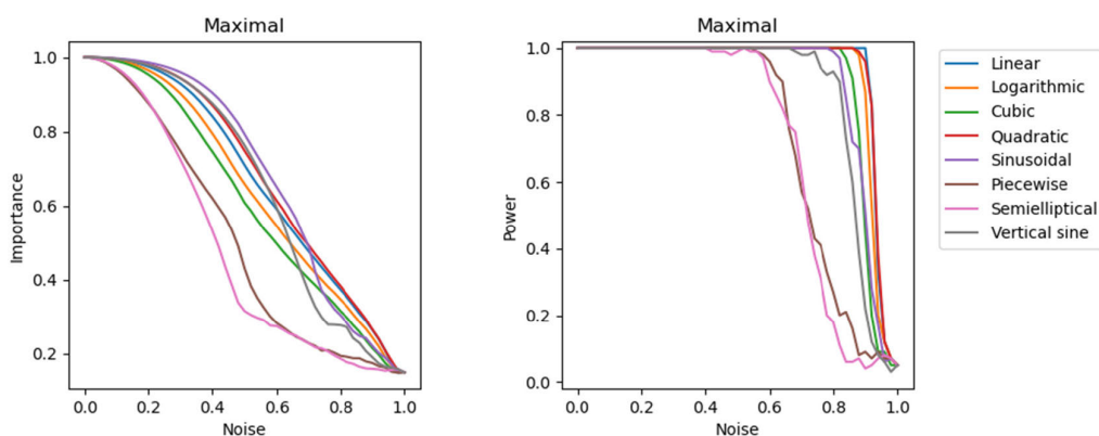
FIGURE 13. Left: Importance based on the maximal correlation coefficient for the synthetic datasets as a function of the noise level ( \beta ). Right: Power of the importance metric.
