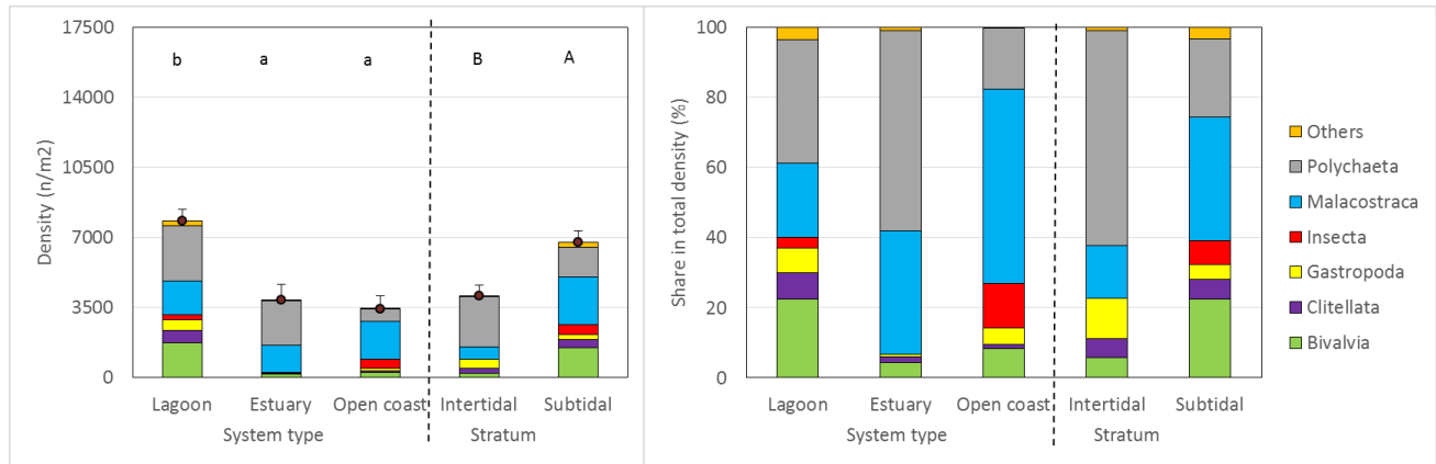
Fig. 11. Absolute (a) and relative (b) numbers of individuals per major taxonomic group for each of the identified system types and strata where sampling has taken place. Average total densities \pm standard error; significant differences in total densities are indicated with different characters where both classification systems (types and strata) have been tested separately as they consist of the same samples.
