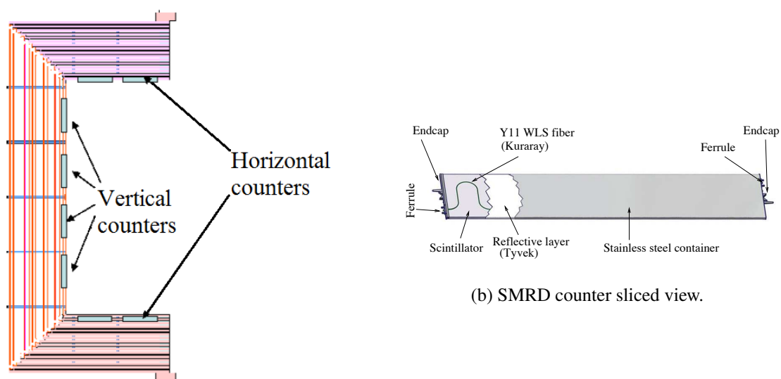
(a) Schematic view of a layer of SMRD modules.
