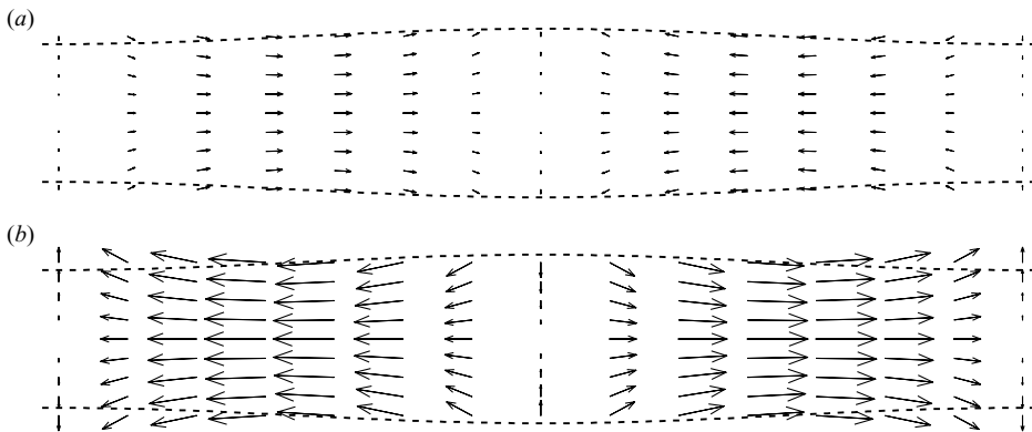
FIGURE 5. Velocity field of the two capillary modes, (a) dominant (b) subdominant, in the zone of aperiodic growth ( C=0.55, k=0.5 ) for the same surface deformation (-·-·).
