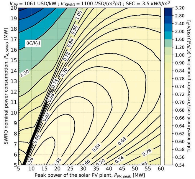
Fig. 14. Total unitary investment cost of the hybrid driven desalination plant - SEC = 3.5 kWh/m 3 .
