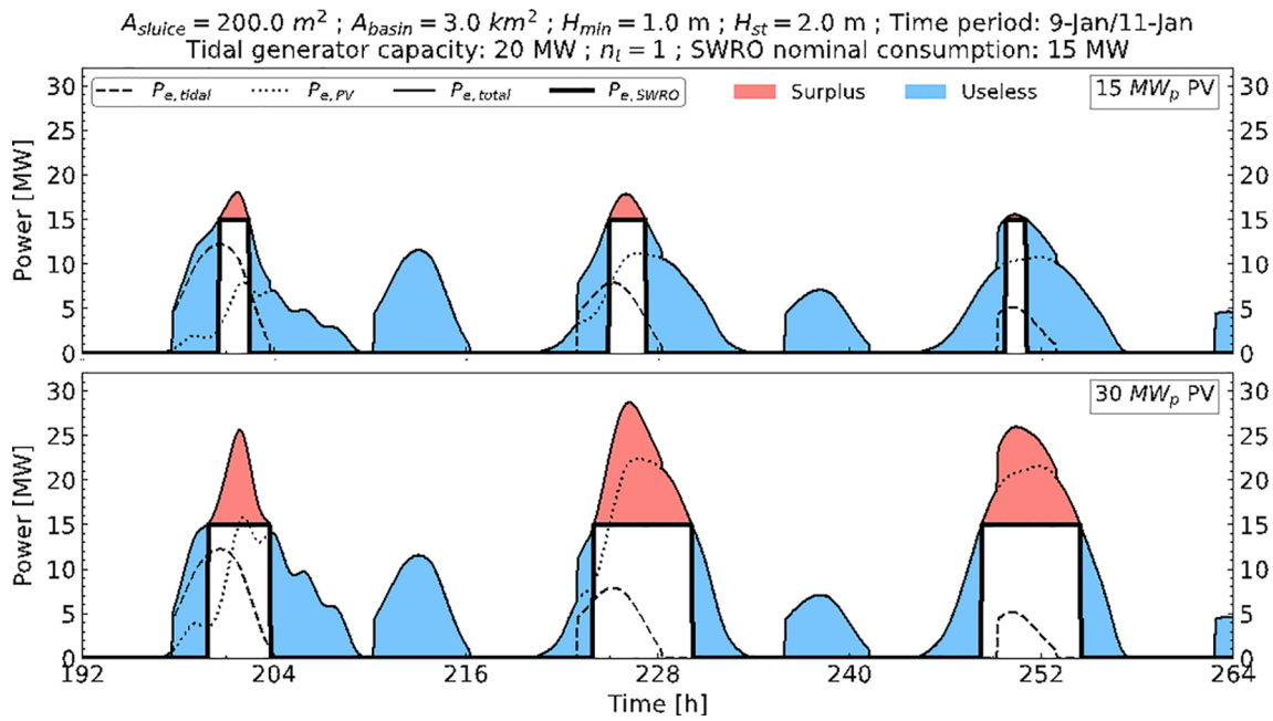
Fig. 6. Power output of the tidal, solar PV and hybrid plants and operation profile of the SWRO plant. No batteries are considered. Case: neap tide period in summer at Broome.
