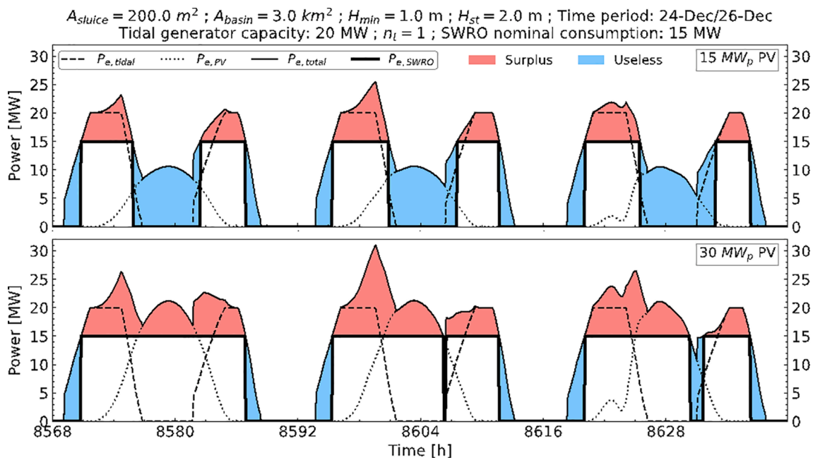
Fig. 5. Power output of the tidal, solar PV and hybrid plant and operation profile of the SWRO plant. Case: spring tide period in summer at Broome.
