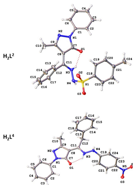
Fig. 3 Molecular structures of ligands \text{H}_2\text{L}^2 and \text{H}_2\text{L}^4 . Thermal ellipsoids are presented at 50% probability.
