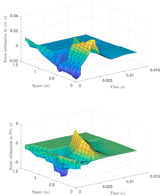
Fig. 1. Estimation error in v(t, x) and P(t, x) as a function of time and space.
