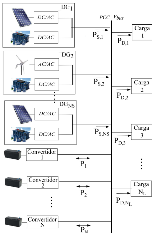
Figura 1: Microrred.
