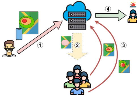
Fig. 1. COVID-Heatmaps app.
