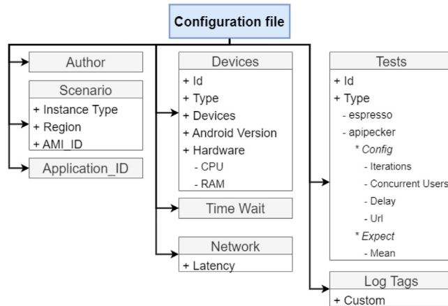
Fig. 3. Conceptual Model. Configuration File.
