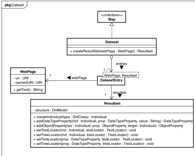
Fig. 1 Dataset Package
