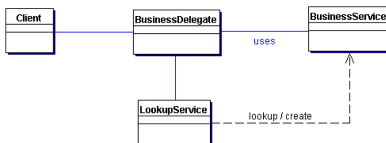
Figura 1. Estructura Business Delegate.
