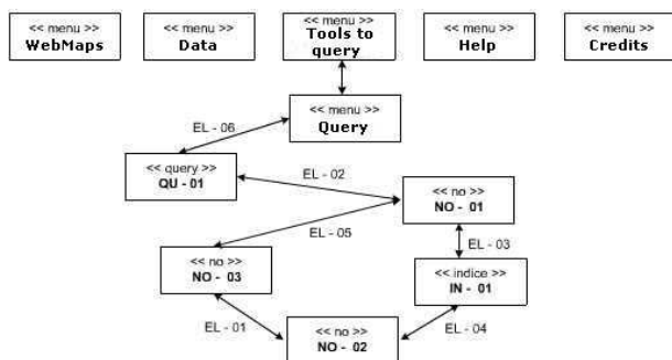
Figure 3. Final navigational model
