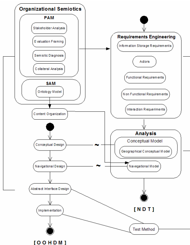
Figure 1. Development process for Web GIS applications (extended)
