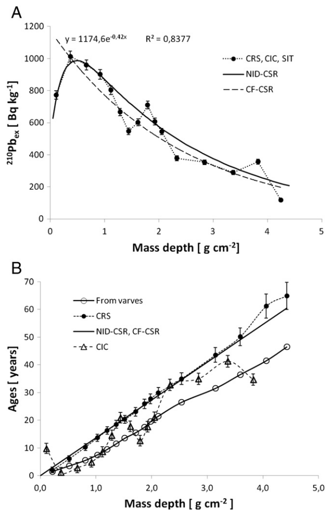
Fig. 5. Example of application of different ^{210}\text{Pb} dating models to a sediment core. (A) Measured (points with error-bars) ^{210}\text{Pb}_{\text{ex}} versus mass depth profile for a sediment core sampled in 1971 in Santa Barbara Basin (from Koide et al., 1973). The exponential fit corresponds to the CF-CSR model while the continuous line is the best fit obtained with the NID-CSR model (parameter values: with \phi = 925 \pm 9 \text{ Bq m}^{-2} \text{ yr}^{-1} , w = 0.073 \pm 0.001 \text{ g cm}^{-2} \text{ yr}^{-1} , g = 0.61 \pm 0.04 and \alpha = 4.2 \pm 0.5 \text{ g}^{-1} \text{ cm}^2 ). Models CRS and CIC are “mapping” models, contained as particular cases of the SIT model. (B) Chronologies produced with the previous models, compared against the one from varve counting (from Koide et al., 1973). Error bars correspond to 1\sigma propagated uncertainties.
