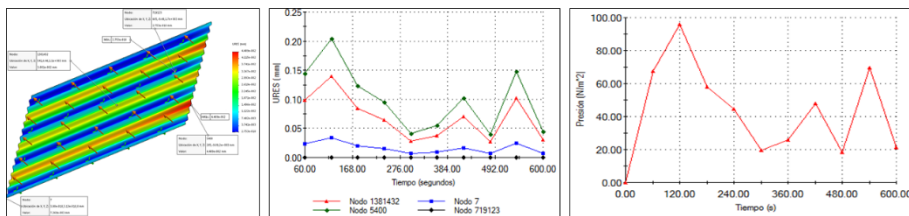
Figure 3. Stress distribution in a lightweight metal roof as a function of time, and the pressures in this type of roof. Source: own elaboration.
