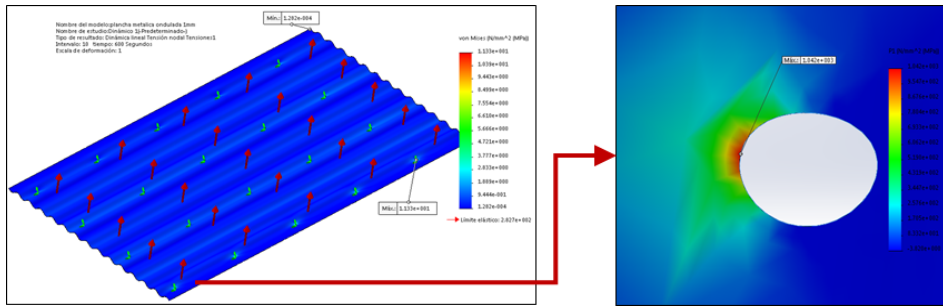
Figure 2. Deformations at the edges of the fixing holes of the metallic light roofs. Source: own elaboration.
