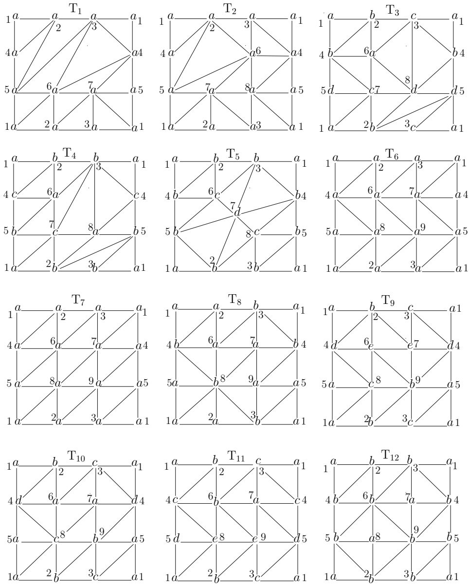
Figure 2. The vertex orbits (to be continued).
