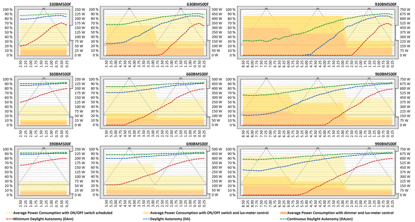
Fig. 6. Analysis of room depth: Room models for Madrid location with variable depth and window size and requirements for full-time frame at 500 lx. The primary Y-axis shows the percentage obtained for the three dynamic metrics, while the secondary Y-axis shows the average power consumption for each of the three solutions of the systems proposed.
