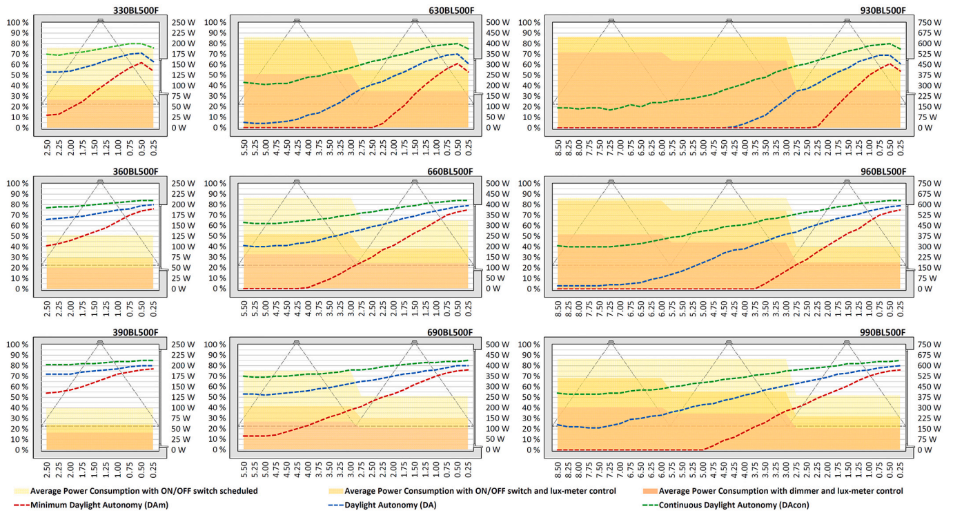
Fig. 7. Analysis of window size: Room models for London location with variable depth and window size and requirements for full-time frame at 500 lx. The primary Y-axis shows the percentage obtained for the three dynamic metrics, while the secondary Y-axis shows the average power consumption for each of the three solutions of the systems proposed.
