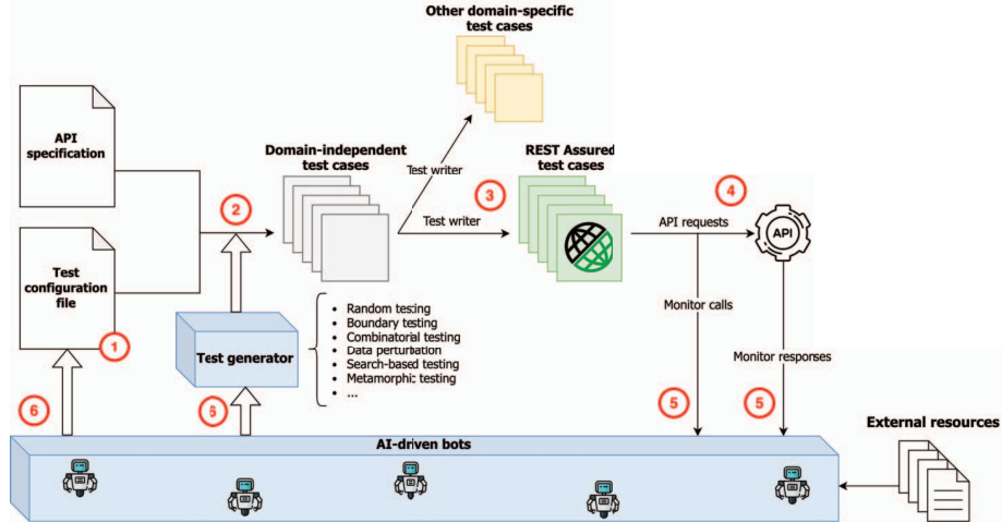
Figure 1: High level architecture of the testing framework.
