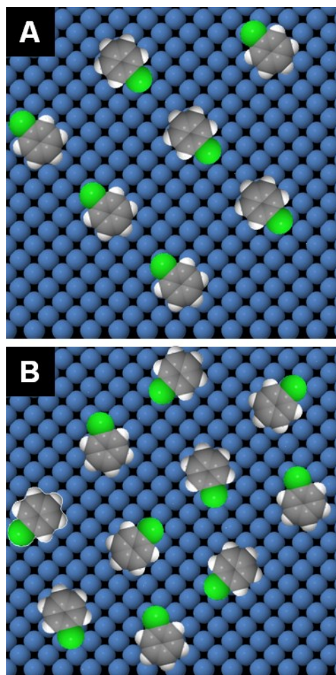
Figure 3. Schematic representation of plausible ClBz structures. Molecules have been represented by their vdW radii. A: rectangular phase. B: hexagonal phase. Color code: green (chlorine), gray (carbon), white (hydrogen) and blue (silver).
