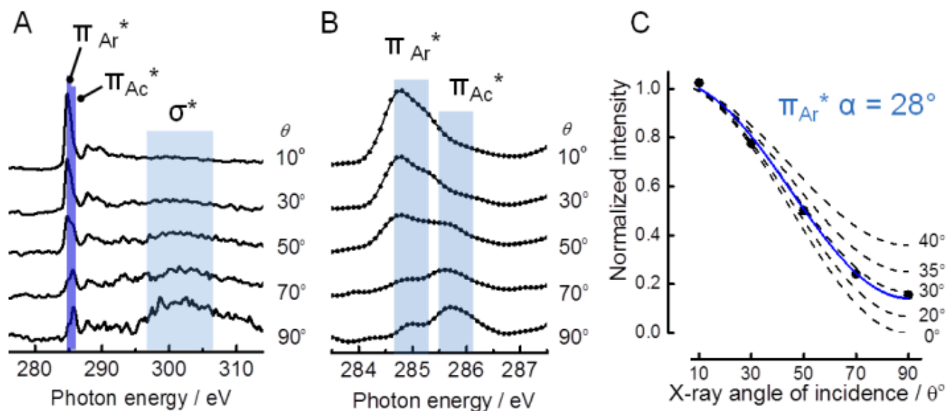
Figure 6. A: C K-edge NEXAFS spectra acquired at five angles of photon incidence \theta for a \sim 1.0 ML coverage of PA on Ag(100) at 170 K. B: Leading \pi^* resonances, expanded scale (Ar = aromatic; Ac = Acetylenic). C: Curve fitting analysis of q dependence of \pi^* resonance A to estimate the phenyl ring tilt angle, \alpha .
