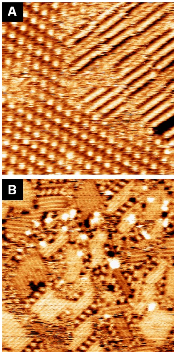
Figure 4. STM images showing progressive formation of biphenyl with increasing temperature. A : 25.0 nm x 25.0 nm) I=0.44 nA V=2.1 V, following further annealing (Si diode temperature = 240 K). B : 25.0 nm x 25.0 nm, I=0.38 nA V=2.1 V following annealing to higher temperature (Si diode temperature = 295 K).
