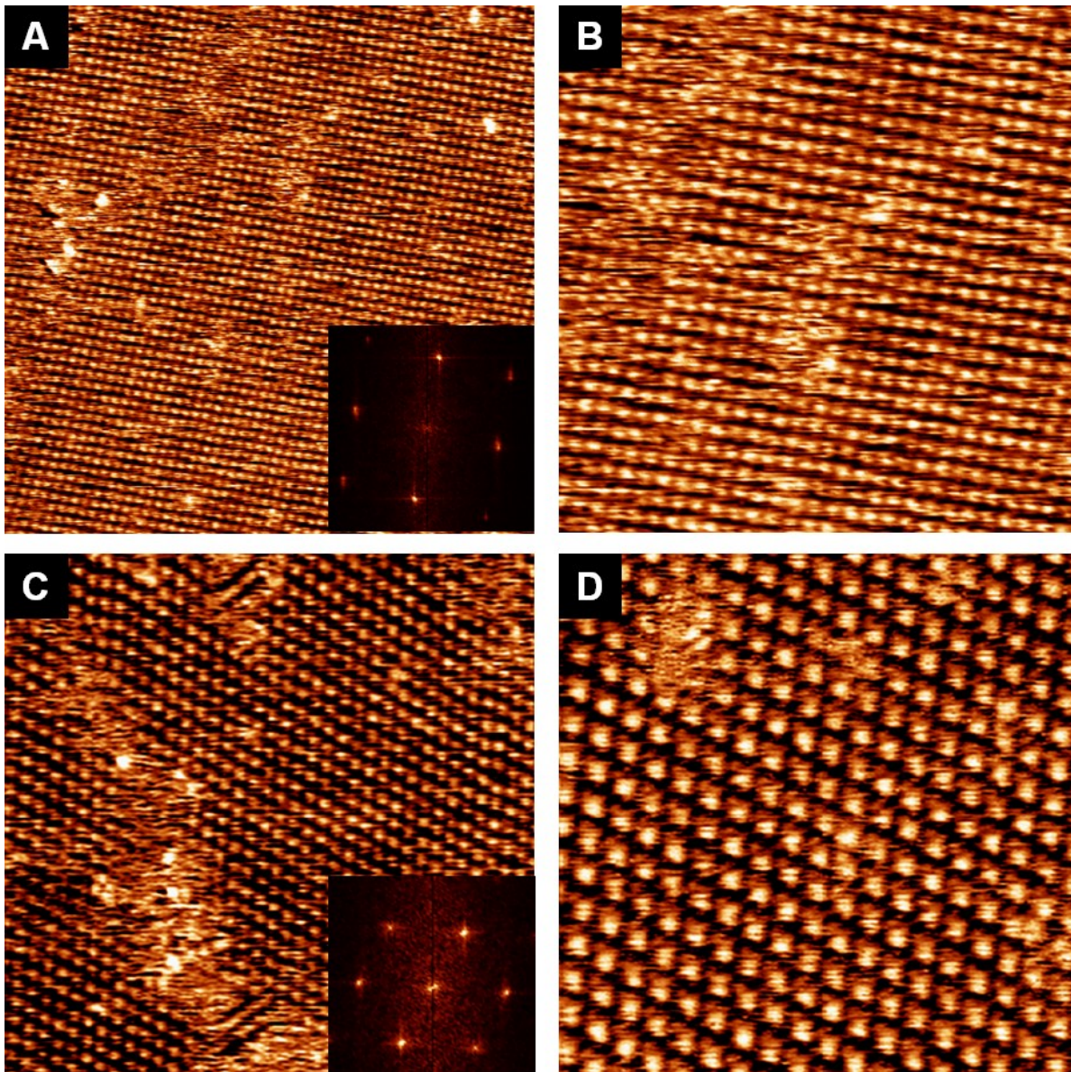
Figure 1. STM images of two different chlorobenzene phases co-existing on the Ag(100) surface after gentle annealing (Si diode temperature = 240 K). Exposure: 2 L. A: STM image of the rectangular phase. Inset: fast Fourier transform of the STM image. STM parameters: (75nm x 75nm) I=0.65 nA V=1.76 V. B: Higher magnification image of the rectangular phase. Each bright feature corresponds to a CIBz molecule. STM parameters: (40.0 nm x 40.0 nm) I=0.65 nA V=1.76 V. C: STM image of the hexagonal phase. Inset: fast Fourier transform of the STM image. STM parameters: (50 nm x 50 nm) I=0.65 nA V=1.76 V. D: Higher magnification image of the hexagonal structure. Each bright feature corresponds to a CIBz molecule. STM parameters: (25 nm x 25 nm) I=0.44 nA V=1.94 V.
