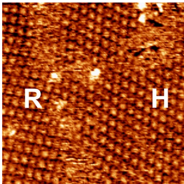
Figure 2. STM image of ClBz on Ag(100) after gentle annealing (Si diode temperature = 240 K), showing coexistence of rectangular ( R ) and hexagonal ( H ) phases. STM parameters: (30 nm x 30 nm) I=0.27 nA V=1.94 V.
