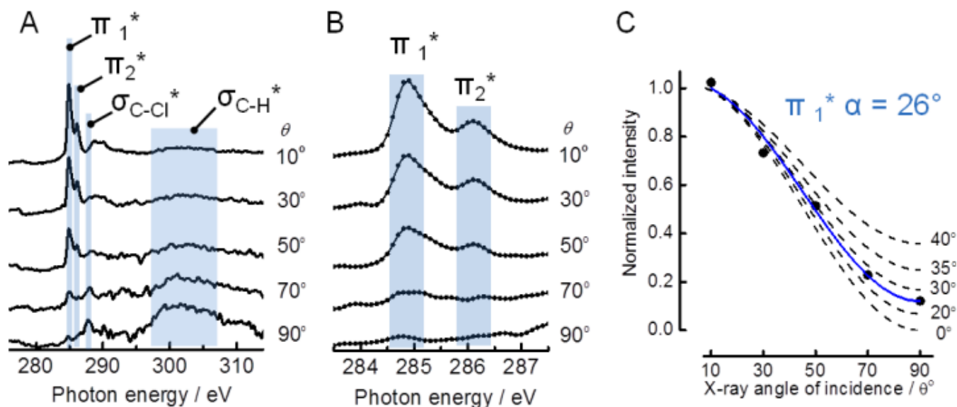
Figure 7. A: C K-edge NEXAFS spectra acquired at five photon incidence angles \theta for a \sim 1.0 ML coverage of ClBz on Ag(100). B: Principal \pi^* resonances expanded scale. C: Curve-fitting analysis of the photon angle dependence of \pi_1^* resonance to estimate the corresponding phenyl ring tilt angle, \alpha .
