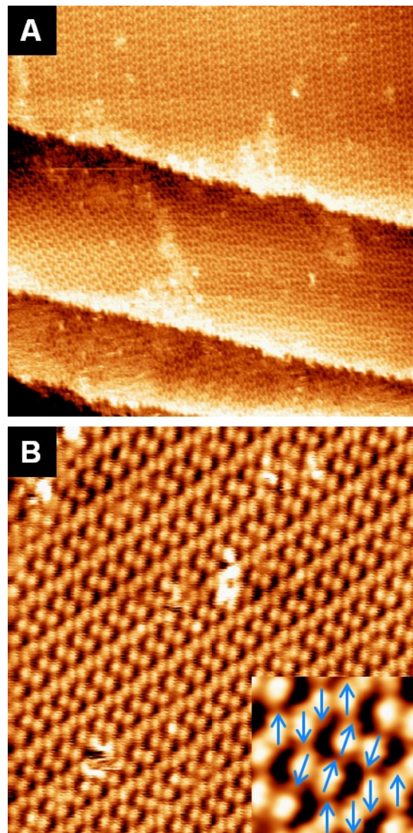
Figure 5. Phenylacetylene island growth on Ag(100). See text. Exposure: 4L. A : (75 nm x 75 nm) I=0.31 nA V=1.89 V. B : (25 nm x 25 nm) I=0.40 nA V=2.31 V. Inset: Magnified image with a superimposed dipole model illustrated as blue arrows.
