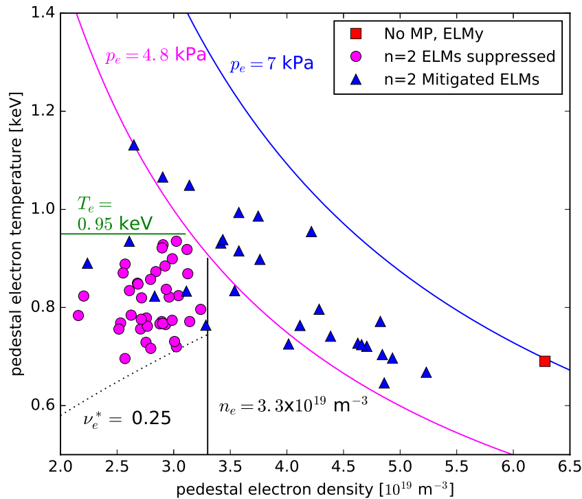
Figure 15. Operational boundaries in pedestal T_e - n_e space of ELM suppression (circles), ELMs H-mode with MP-mitigated small ELMs (triangles), and ELMs H-mode with MP off (red square).
