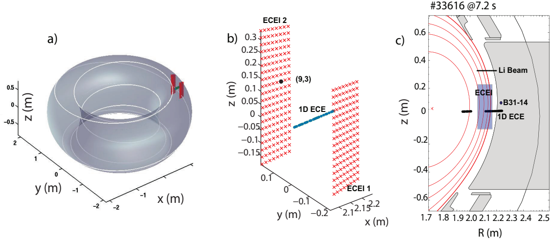
Figure 1: a) q = 6 flux surface plotted as a gray shaded area for the shot # 33616 at t 7.2 s. Magnetic field line for this equilibrium is plotted as white solid line. The red surfaces, intersecting the q = 6 flux tube correspond to two ECEI imaging systems. b) Absolute measurement positions of two toroidally separated ECEI arrays in Cartesian coordinates are shown as red crosses (X); edge channels of conventional ECE radiometer are shown as green dots. The ECEI channel of the ECEI 2 array that is used for comparison with the magnetic measurements is marked as black circle (●). c) Poloidal cross section of ASDEX Upgrade indicating the measurement positions of: the Lithium beam diagnostic, ECE Imaging, standard ECE radiometer and magnetic pick-up coil (B31-14).
