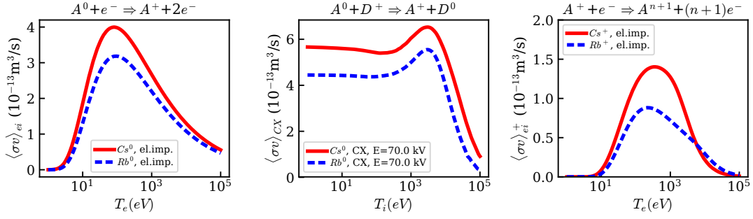
Figure 2. Rate coefficients for the atomic species A = \text{Cs} and A = \text{Rb} . Left: electron impact ionization of neutral atoms. Middle: charge-exchange collisions with Deuterium. Right: electron impact ionization of singly ionized ions.
