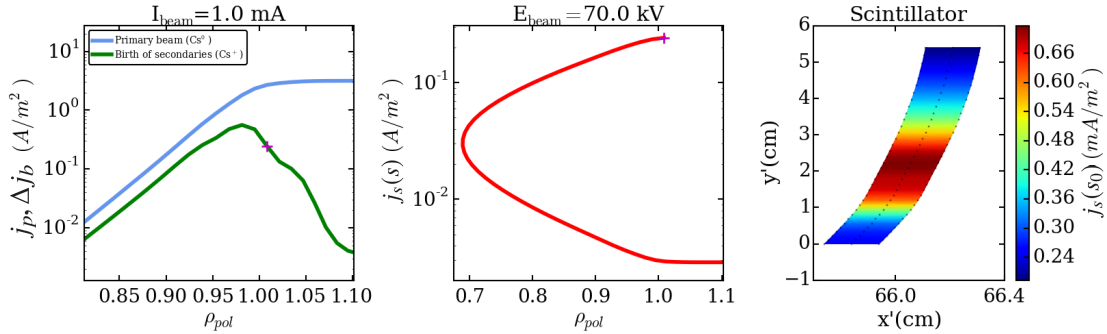
Figure 3. Left: attenuation of primary beam j_p and birth profile of secondaries \Delta j_b versus normalized poloidal flux coordinate \rho_{pol} . Middle: attenuation of secondary beam current density j_s . Right: ion flux pattern and intensity on scintillator. y' and x' are the vertical and horizontal coordinates on the scintillator plate.
