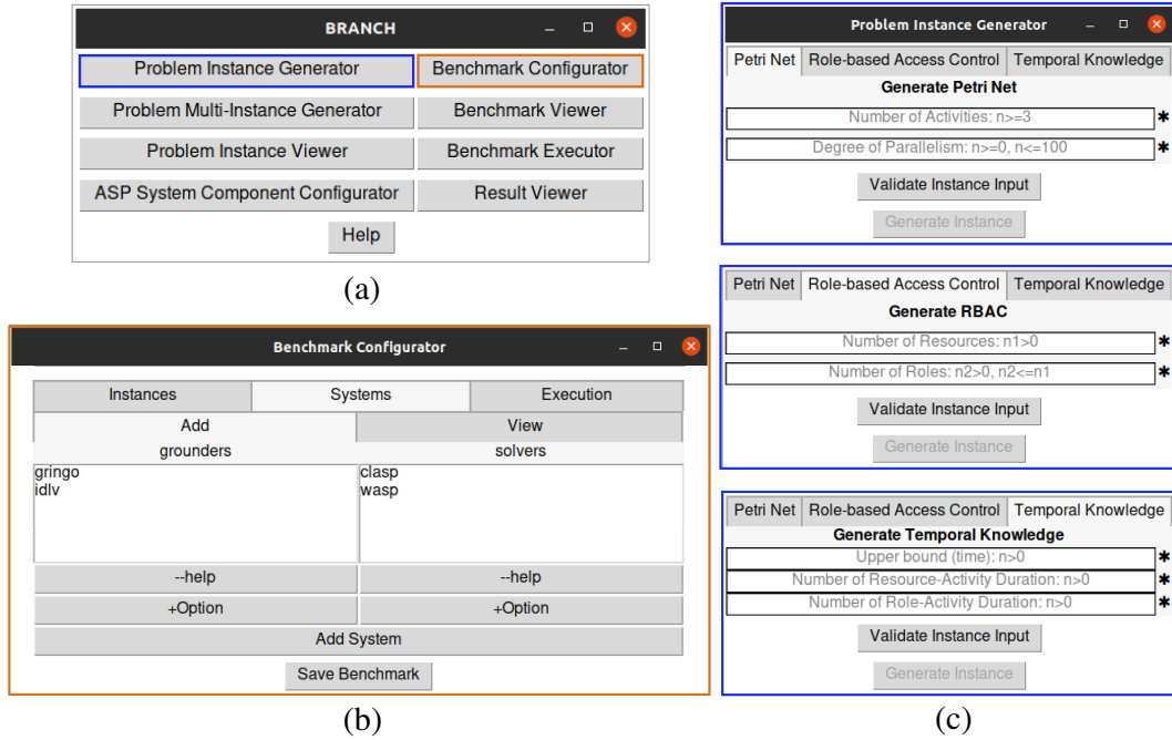
Figure 1: Screenshots of BRANCH
