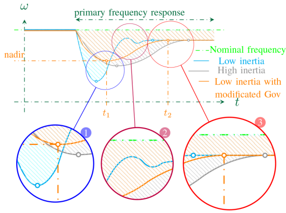
Fig. 7 Power system frequency response: Optimisation regions
