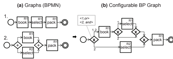
Figure 4: Two BP graphs (a) are merged into a single configurable BP graph (b).
