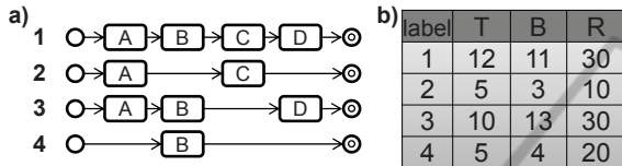
Figure 6: (a) Different BP models. (b) Table of BP model properties.
