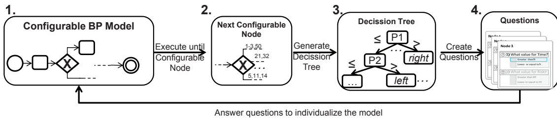
Figure 5: The proposed method.
