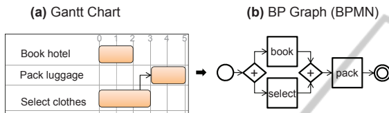
Figure 3: A schedule (a) as a BP Graph (b).
