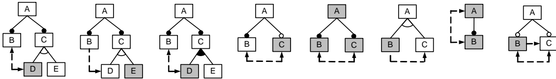
Figure 4: Input feature models with dead features (grey features are dead)
