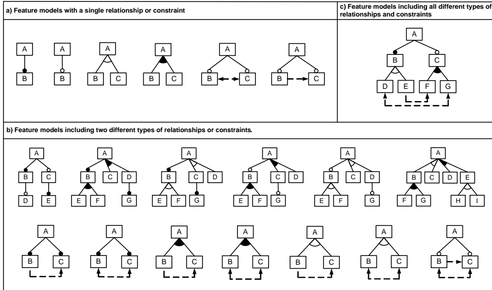
Figure 2: Equivalence partitions on feature models
