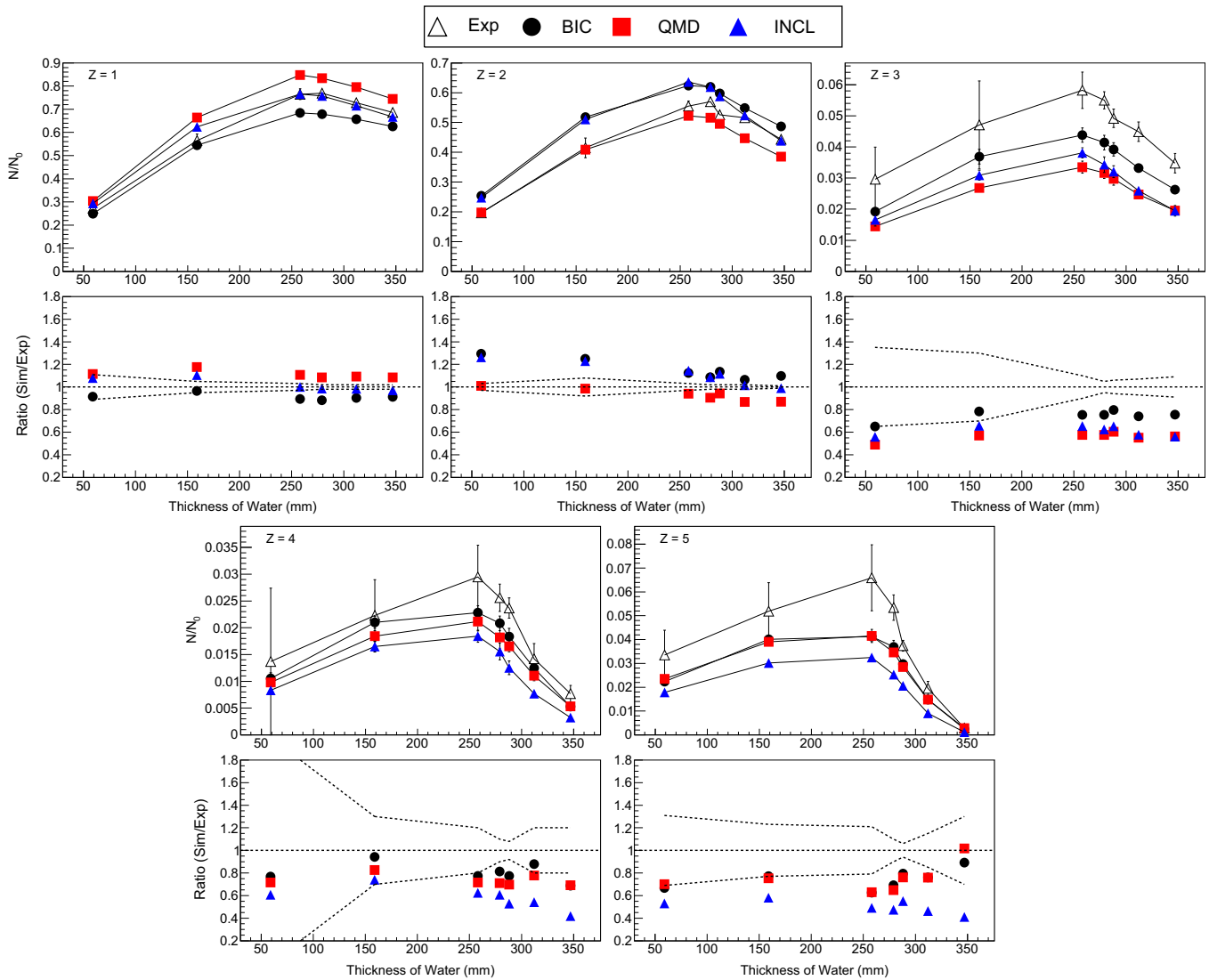
FIG. 19. The fragment yields, N , produced from N_0 monoenergetic 400 MeV/u 12 C ions incident upon different thicknesses of water. The fragments were scored within a forward angle of 10° from the center of the water targets. Experimental measurements of fragments with different atomic number ranging from 1 to 5 are compared against alternative models available in Geant4. The dashed lines on the bottom ratio plots indicate the experimental uncertainty \sigma_{ref} . [Color figure can be viewed at wileyonlinelibrary.com]
