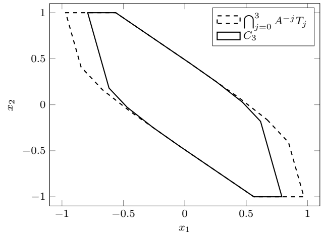
Fig. 1. Comparison of C_3 and its bounding set \bigcap_{j=0}^3 A^{-j} T_j for system \mathbf{S}_3 with \alpha = 0.1 .
