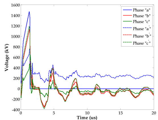
Fig. 15 Overvoltage of different conductors – 83 kA lightning – two shield wires
