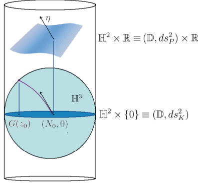
Figura 1: The hyperbolic Gauss map for surfaces in \mathbb{H}^2 \times \mathbb{R} .
